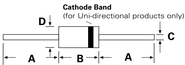
DO-204AC (DO-15)
